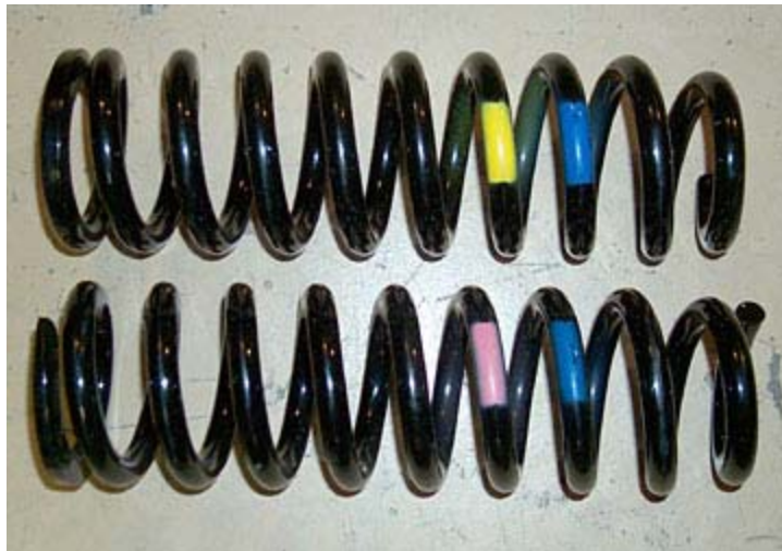
Left and Right 1999 front coils. V6, 4WD and 16" wheel truck.
